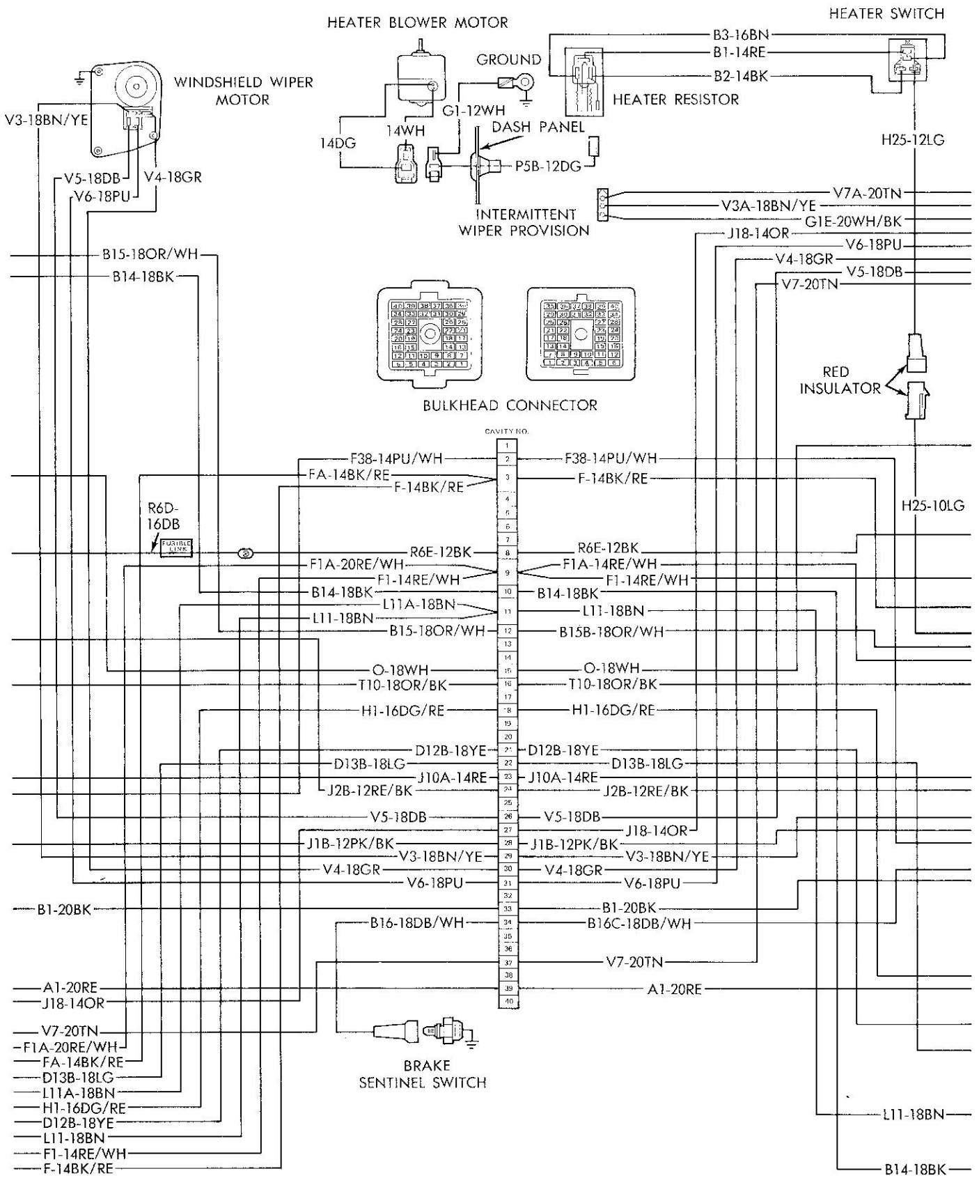
Fig. 1—Complete Vehicle Wiring Diagrams
