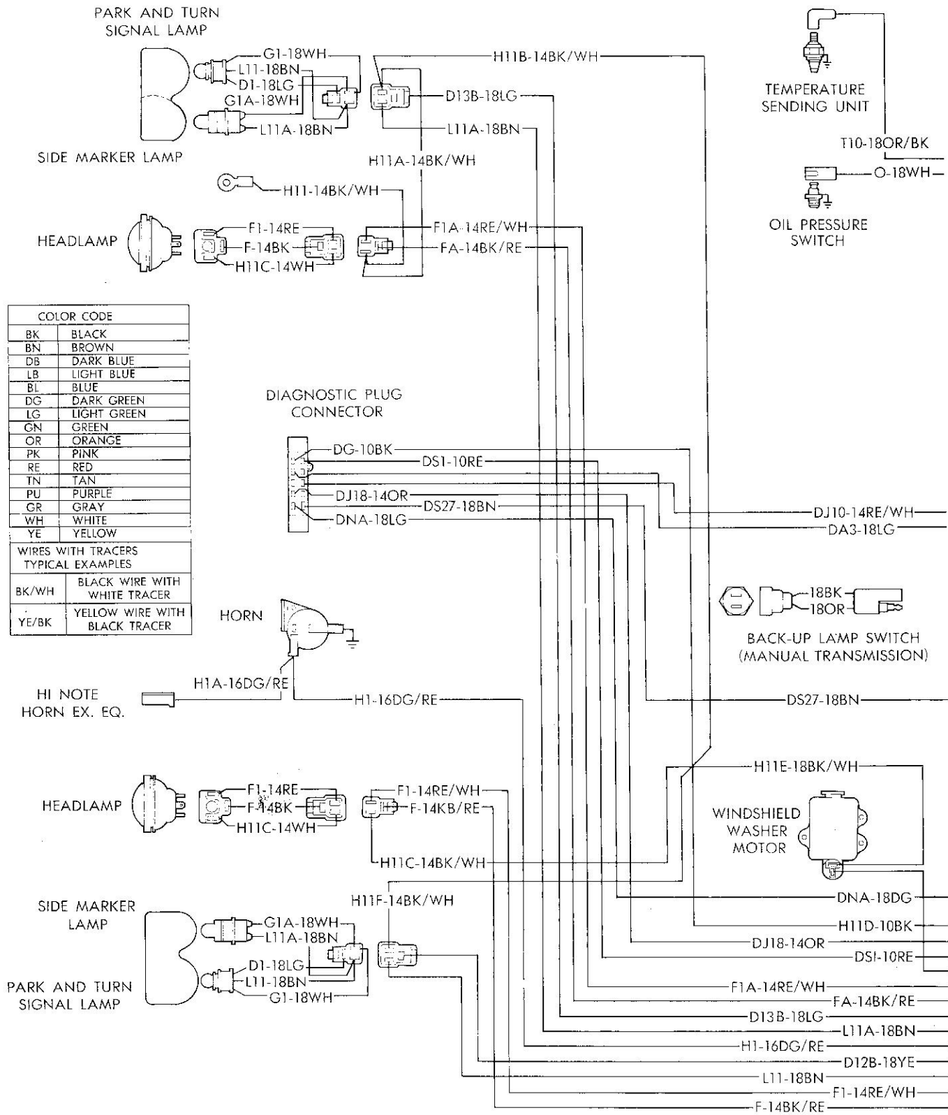
Fig. 1—Complete Vehicle Wiring Diagrams
